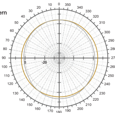
E-Plane Pattern
